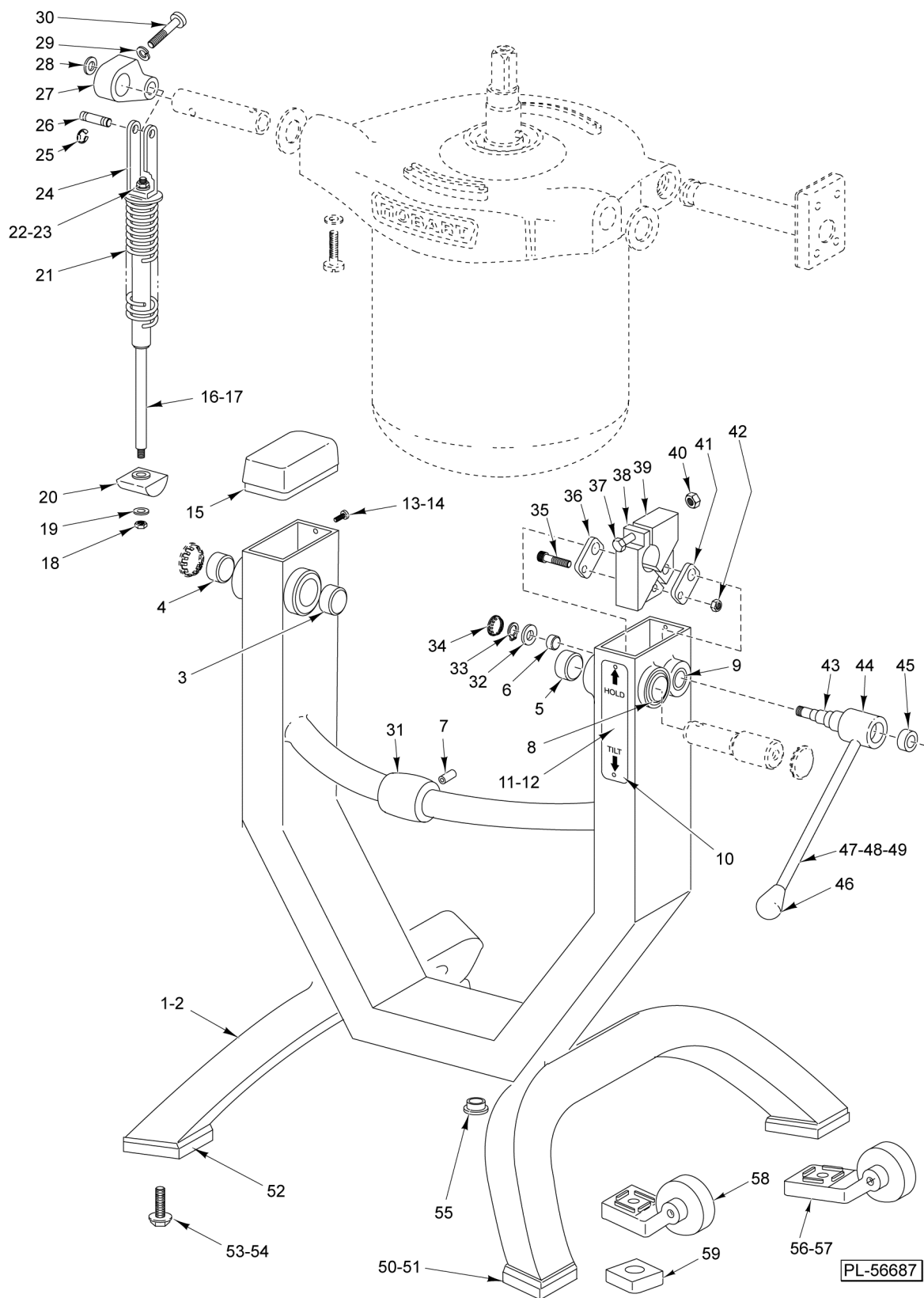
FRAME ASSEMBLY
